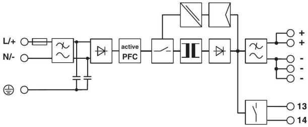
Figure 2 Block diagram
