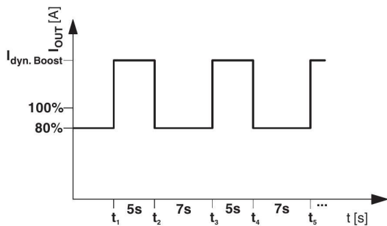
Figure 17 Schematic diagram of dynamic boost behavior
