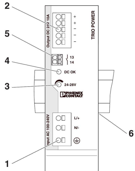
Figure 3 Function elements
