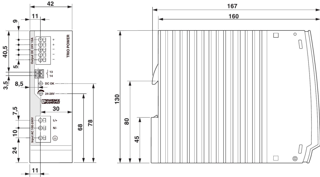
Figure 6 Device dimensions
